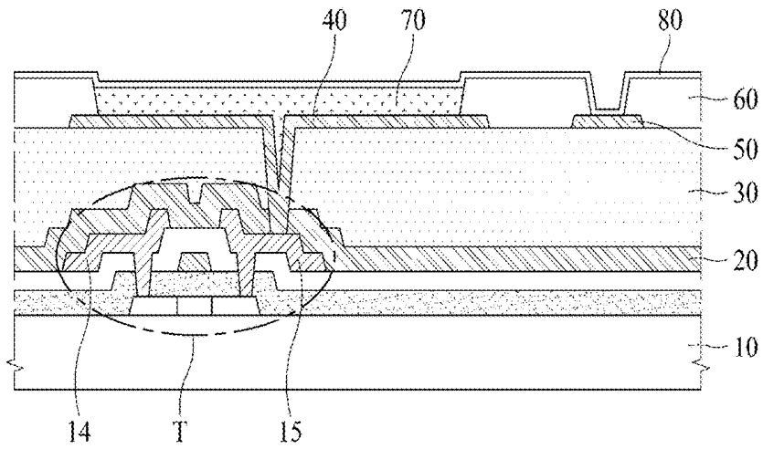
FIG.1 RELATED ART
